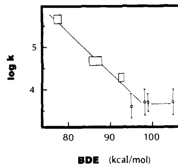
Figure 8. Correlation of the rates of fragmentation of benzoate radical anions \text{R}-\text{OCOC}_6\text{H}_5^{\bullet-} ( \log k ) with bond dissociation energies (BDE) of corresponding R—H bonds.
