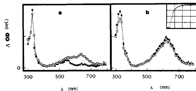
Figure 3. Difference transient absorption spectra of benzophenone determined 0.5 (circles) and 67 \mu s (triangles) after a 100-ns pulse of electrons (a) in alcohol and (b) in alcohol containing 0.1 M KOH. Inset shows time dependence (1.9 \mu s/division) of absorption of 640 nm together with first-order fit (solid trace) in the presence of KOH.
