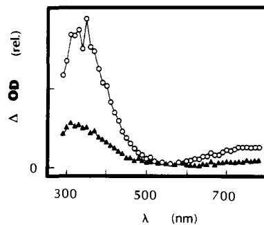
Figure 2. Difference transient absorption spectra of diethyl phthalate in alcohol determined 5 (circles) and 672 \mu s (triangles) after a 100-ns pulse of electrons.
