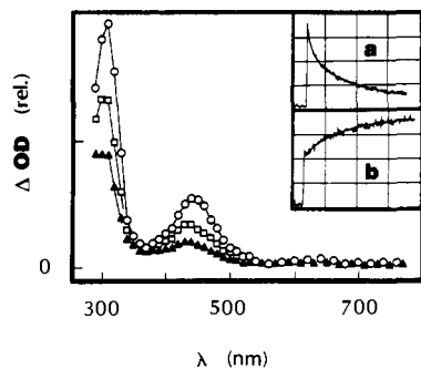
Figure 1. Difference transient absorption spectra of ethyl benzoate in alcohol determined 1 (○), 37 (□), and 135 (▲) \mu s after a 100-ns pulse of electrons. Insets show time dependence of absorption at 450 nm (a) in the absence of added base (110 \mu s/division) and (b) in the presence of 0.1 M KOH (260 \mu s/division), together with exponential fits (solid traces).
